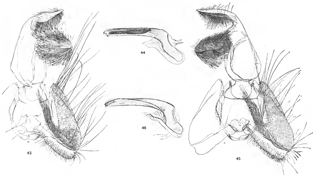
FIG. 43-46. — Male genitalia of Madagascan Tortricinae. 43, Goniotorna (Oestophyes) trigodes sp. nov., paratype, genit. slide 8290 ; 44, the same, aedeagus ; 45, the same, holotype ; 46, the same, aedeagus.
